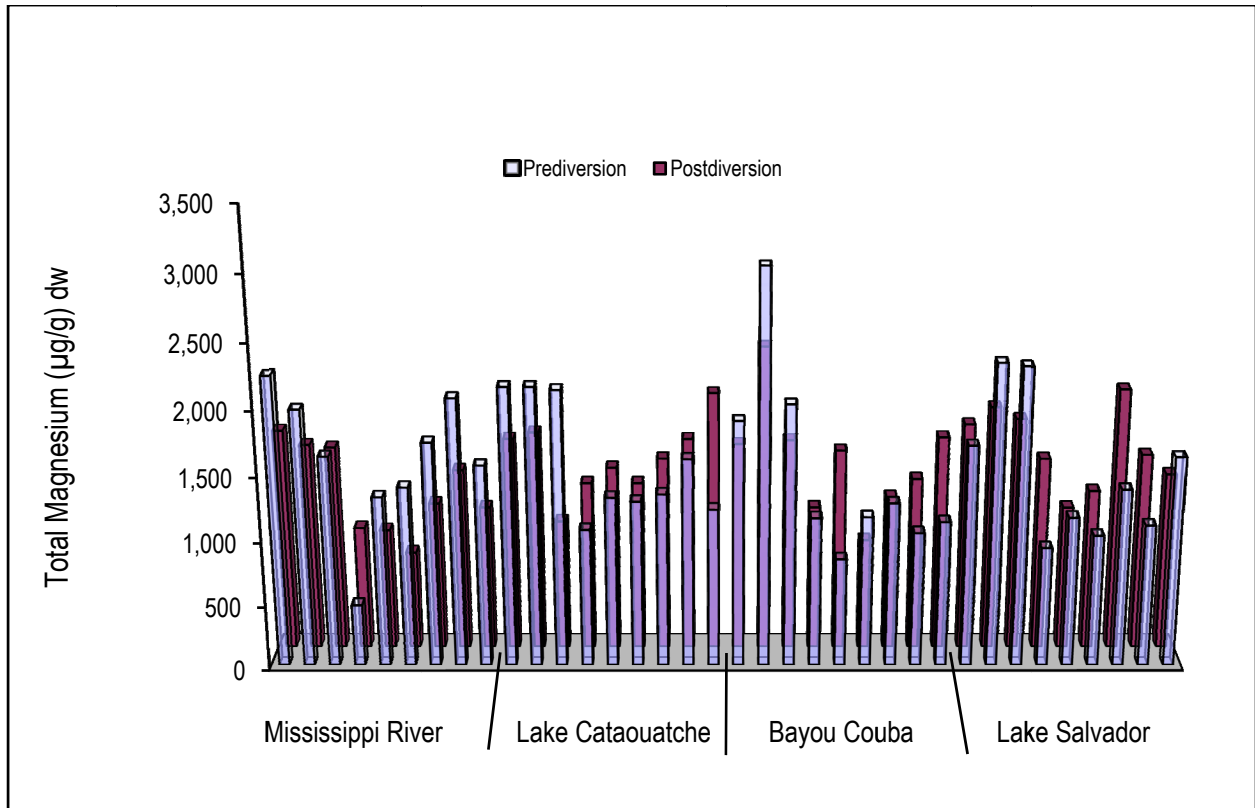
Figure 18B. Three-dimensional comparison of Davis Pond prediversion and postdiversion values for magnesium by dry weight (in micrograms per gram [ \mu\text{g/g} ]).
